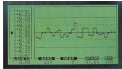
DISTRIBUTION CHARTING
