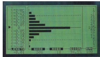
HISTOGRAM
